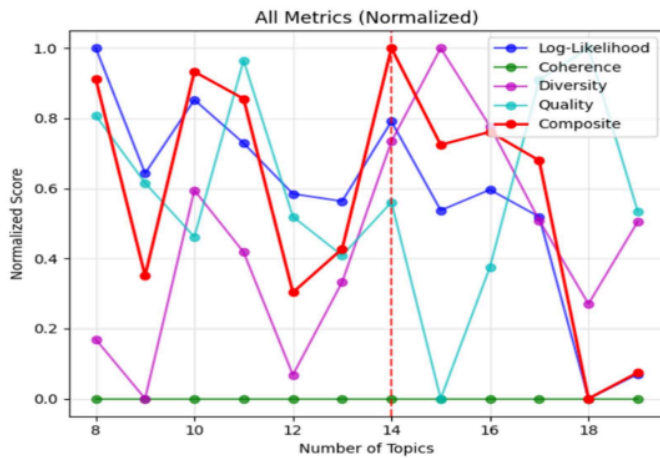
Gambar 4. 7 Grafik Normalized Score vs Number of topics
