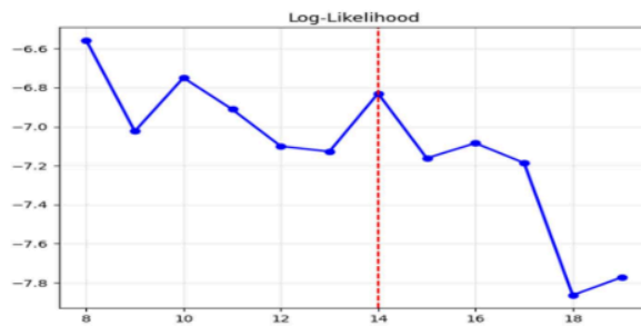
Gambar 4. 2 Grafik Log-Likelihood vs Number of Topics
