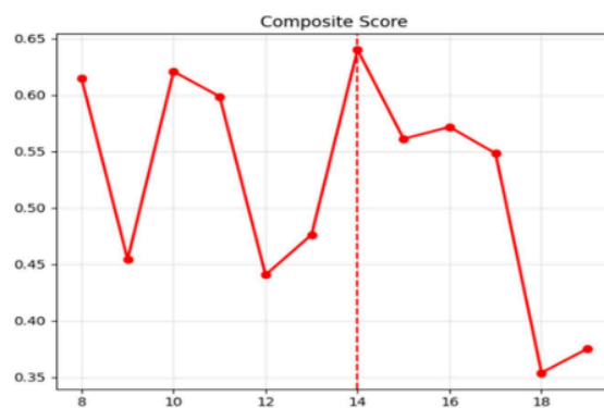
Gambar 4. 6 Grafik Composite Score vs Number of Topics
