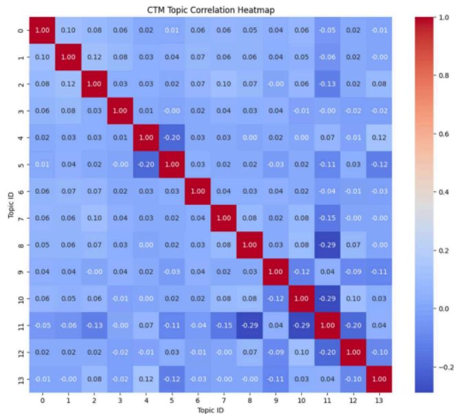
Gambar 4. 8 Grafik CTM Topic Correlation Heatmap
