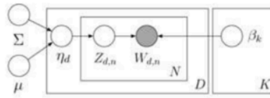
Gambar 2.1 Probabilistic Graphical Model CTM
